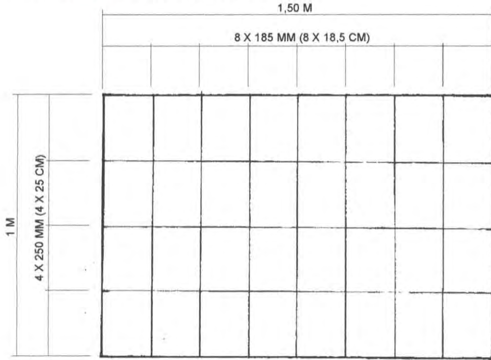
DESPIECE RETAL
