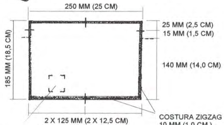
DESPIECE RETAL
